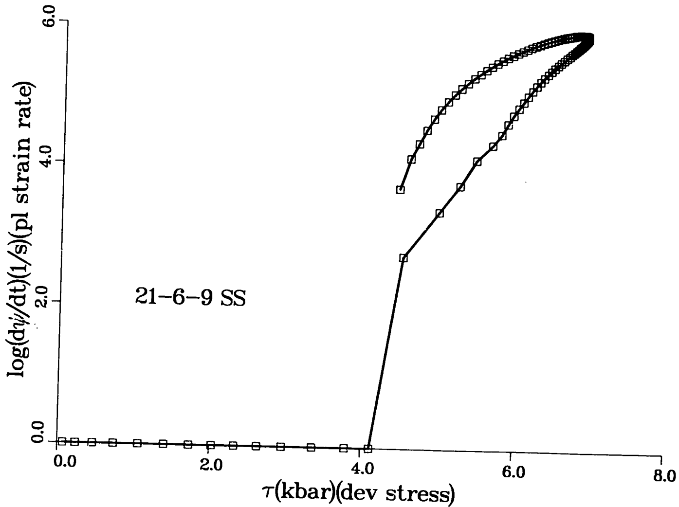
Fig. 43. Log(base 10) of in situ plastic strain rate versus deviatoric stress for shot SSWPIS of 21-6-9 stainless steel. Line is to guide the eye.
