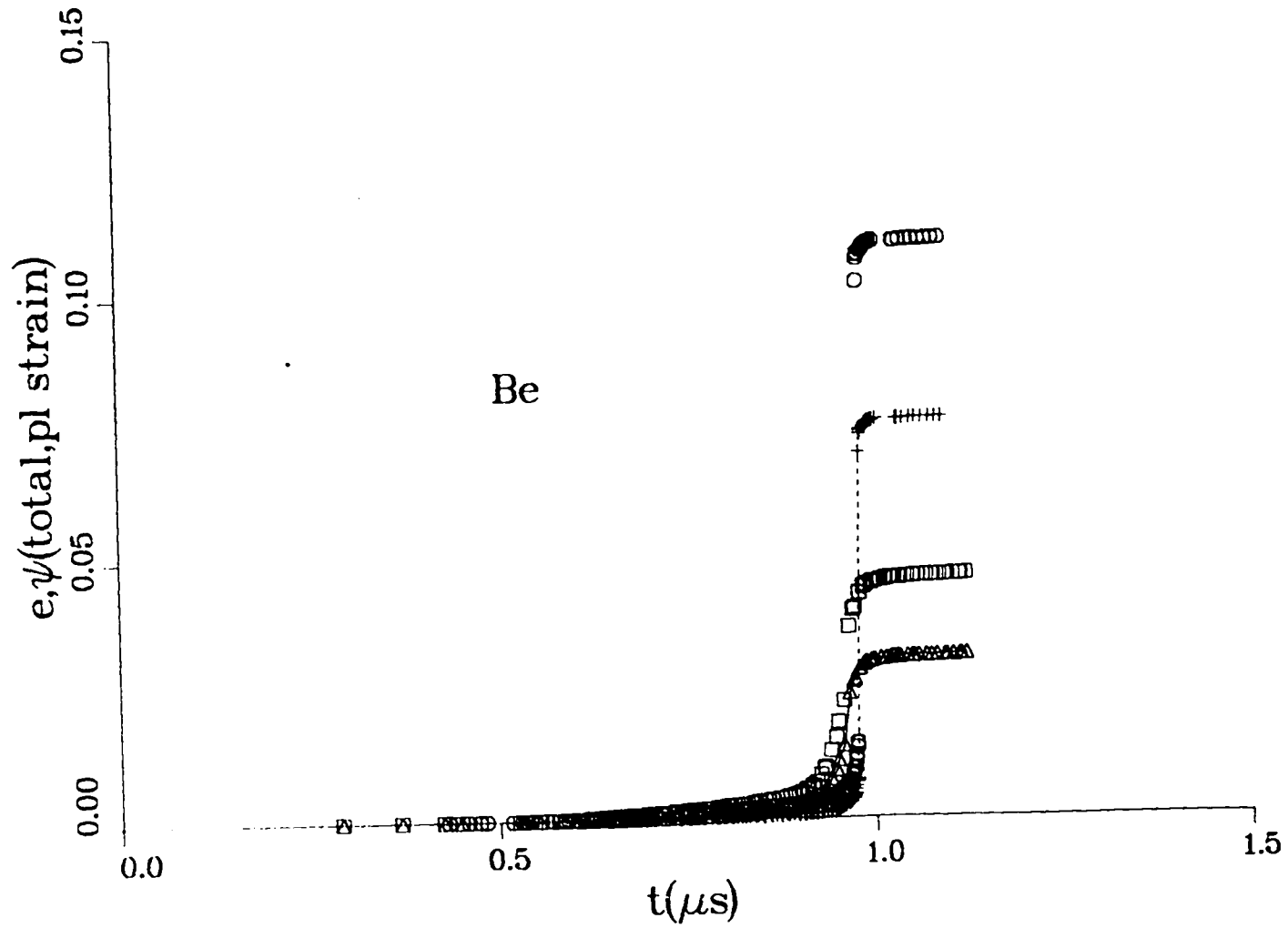
Fig. 10. In situ total strain and plastic strain versus time for beryllium. Squares and circles are total strains for shots Be18 and Be14, respectively. Triangles and pluses are plastic strains for shots Be18 and Be14, respectively. Lines are to guide the eye.
