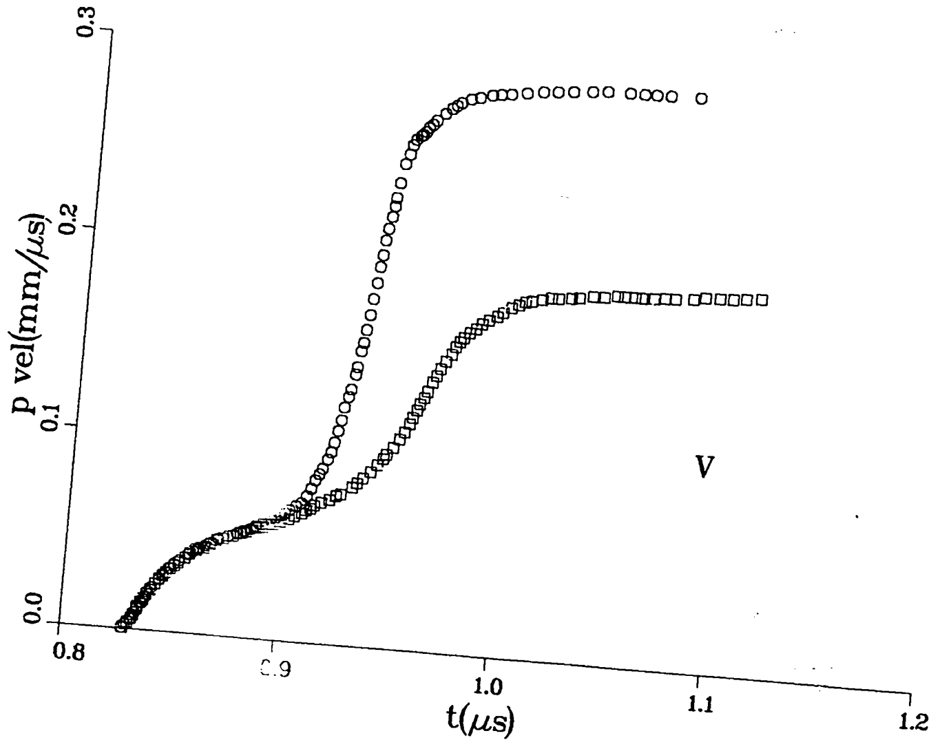
Fig. 51. Particle velocity versus time for vanadium. Squares and circles are for shots VAN2 and VAN3, respectively.
