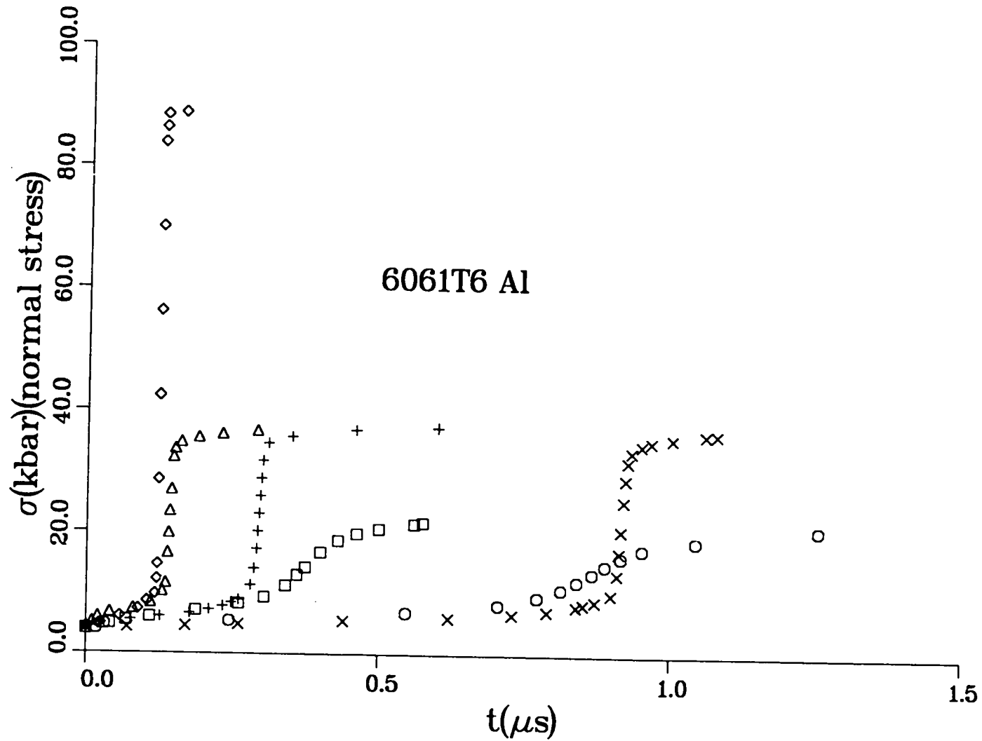
Fig. 4. In situ normal stress versus time for 6061T6 Al. Squares, circles, triangles, crosses, Xs, and diamonds are for shots 922, 939, 936, 927, 937, and 926, respectively.
