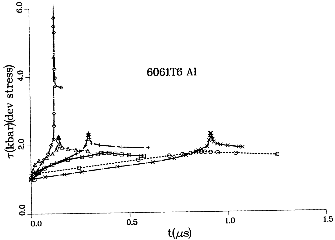
Fig. 5. In situ deviatoric stress versus time for 6061T6 Al. Correspondence between symbols and shots same as for Fig. 4. Lines are to guide the eye.
