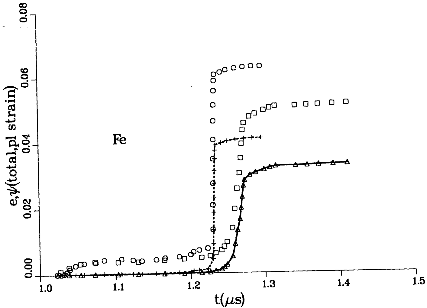
Fig. 31. In situ total and plastic strains for iron. Squares and circles are total strains for shots 15 and 16, respectively. Triangles and pluses are plastic strains for shots 15 and 16, respectively. Lines are to guide the eye.
